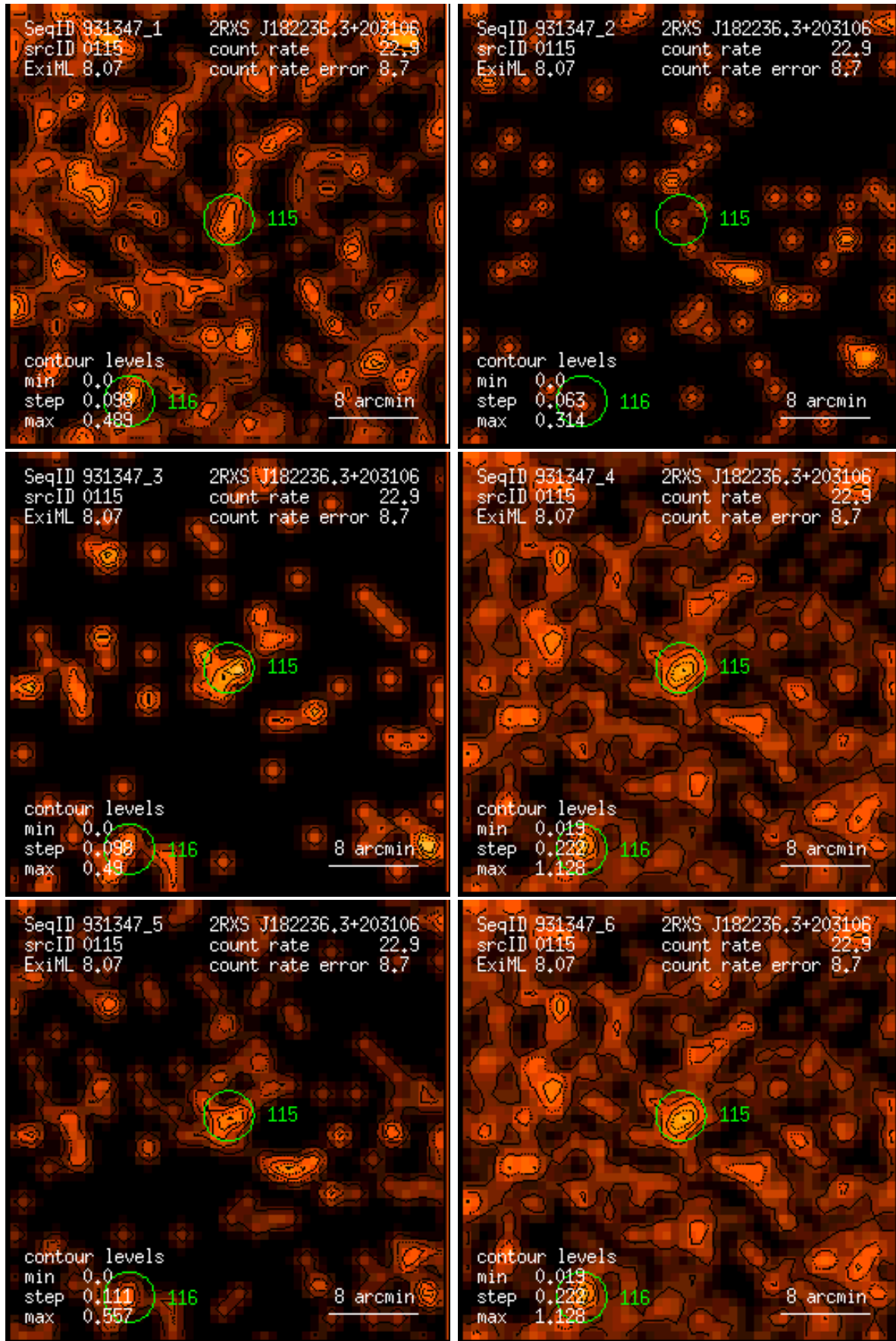
Figure 115: RASS 931347: detection 0115: band rate images, Gaussian filter: (1) PSPC channels 11 – 41, (2) 52 – 90, (3) 91 – 201, (4) 11 – 235, (5) 52 – 201, (6) 11 – 201. Broad band rates in counts/ks. Band rate contour levels in counts/ks/arcmin 2 .
