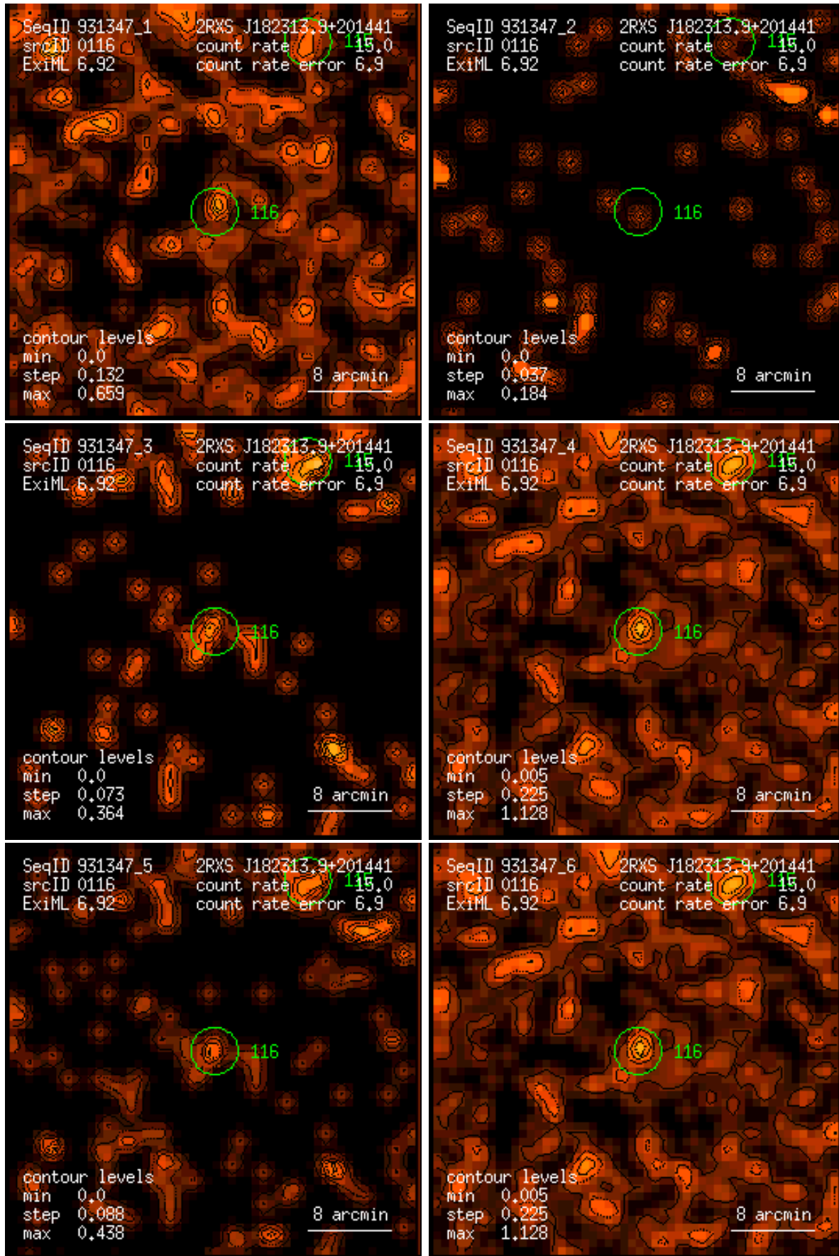
Figure 116: RASS 931347: detection 0116: band rate images, Gaussian filter: (1) PSPC channels 11 – 41, (2) 52 – 90, (3) 91 – 201, (4) 11 – 235, (5) 52 – 201, (6) 11 – 201. Broad band rates in counts/ks. Band rate contour levels in counts/ks/arcmin 2 .
