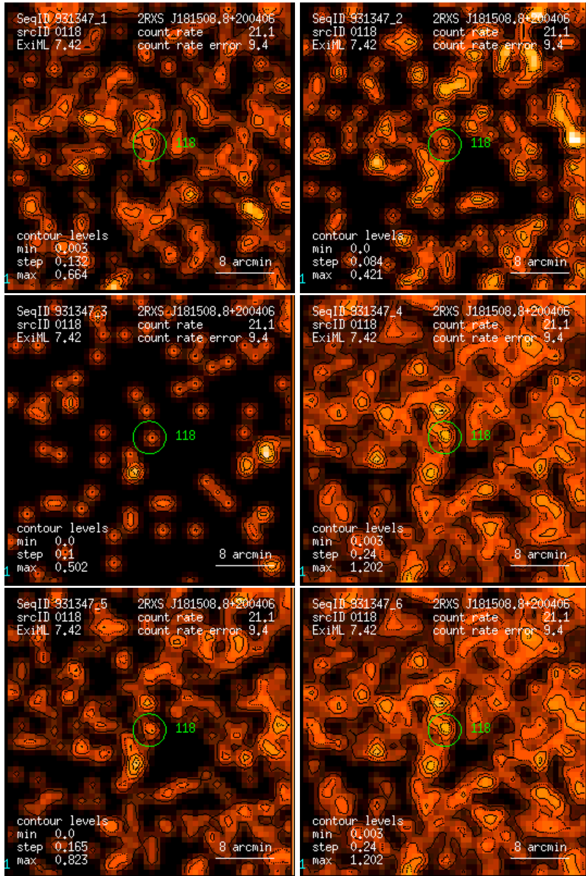
Figure 118: RASS 931347: detection 0118: band rate images, Gaussian filter: (1) PSPC channels 11 – 41, (2) 52 – 90, (3) 91 – 201, (4) 11 – 235, (5) 52 – 201, (6) 11 – 201. Broad band rates in counts/ks. Band rate contour levels in counts/ks/arcmin 2 .
