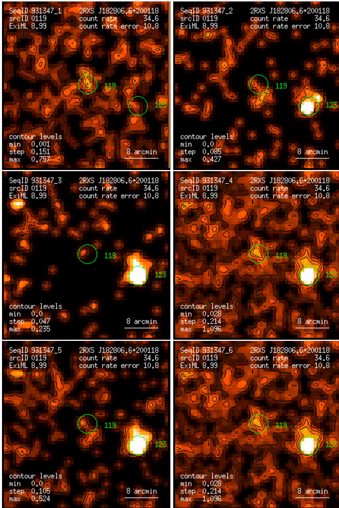
Figure 119: RASS 931347: detection 0119: band rate images, Gaussian filter: (1) PSPC channels 11 – 41, (2) 52 – 90, (3) 91 – 201, (4) 11 – 235, (5) 52 – 201, (6) 11 – 201. Broad band rates in counts/ks. Band rate contour levels in counts/ks/arcmin 2 .
