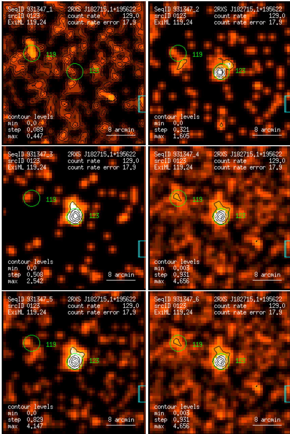
Figure 123: RASS 931347: detection 0123: band rate images, Gaussian filter: (1) PSPC channels 11 – 41, (2) 52 – 90, (3) 91 – 201, (4) 11 – 235, (5) 52 – 201, (6) 11 – 201. Broad band rates in counts/ks. Band rate contour levels in counts/ks/arcmin 2 .
