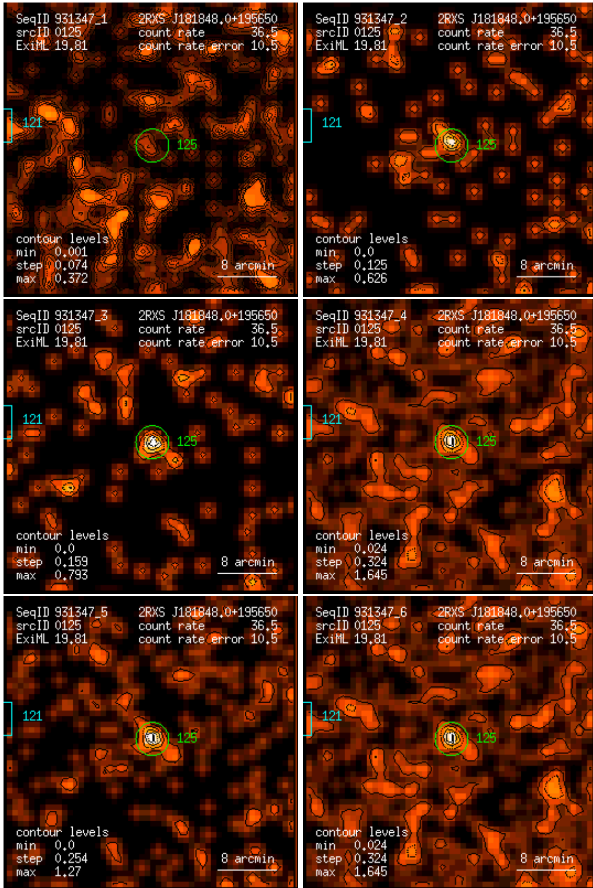
Figure 125: RASS 931347: detection 0125: band rate images, Gaussian filter: (1) PSPC channels 11 – 41, (2) 52 – 90, (3) 91 – 201, (4) 11 – 235, (5) 52 – 201, (6) 11 – 201. Broad band rates in counts/ks. Band rate contour levels in counts/ks/arcmin 2 .
