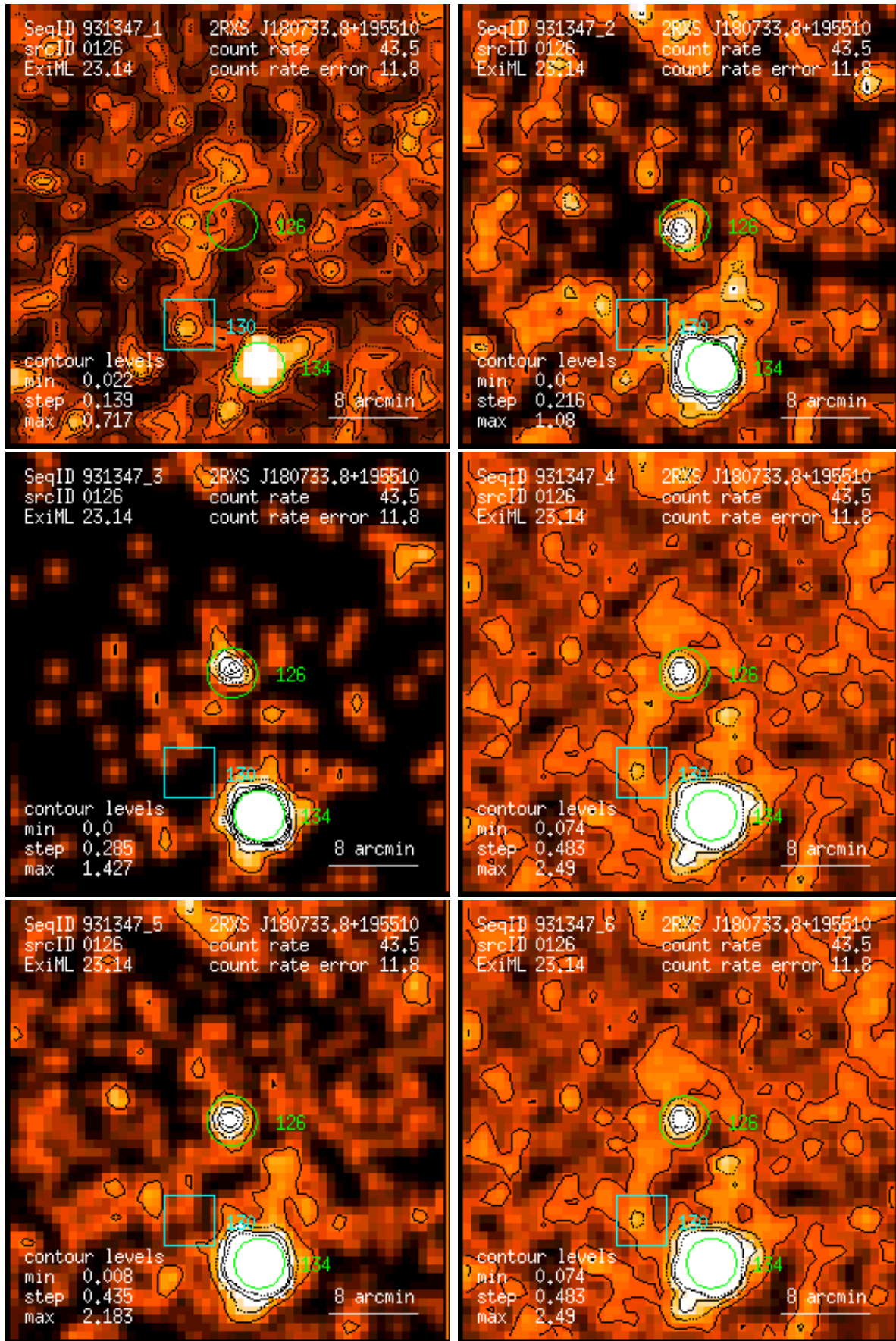
Figure 126: RASS 931347: detection 0126: band rate images, Gaussian filter: (1) PSPC channels 11 – 41, (2) 52 – 90, (3) 91 – 201, (4) 11 – 235, (5) 52 – 201, (6) 11 – 201. Broad band rates in counts/ks. Band rate contour levels in counts/ks/arcmin 2 .
