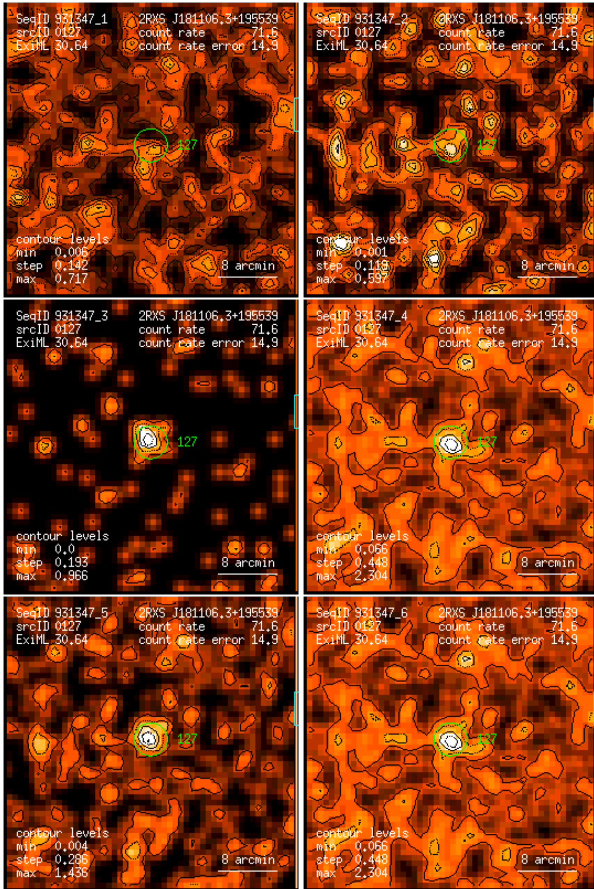
Figure 127: RASS 931347: detection 0127: band rate images, Gaussian filter: (1) PSPC channels 11 – 41, (2) 52 – 90, (3) 91 – 201, (4) 11 – 235, (5) 52 – 201, (6) 11 – 201. Broad band rates in counts/ks. Band rate contour levels in counts/ks/arcmin 2 .
