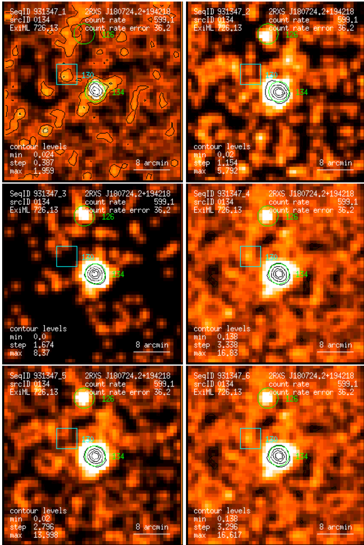
Figure 134: RASS 931347: detection 0134: band rate images, Gaussian filter: (1) PSPC channels 11 – 41, (2) 52 – 90, (3) 91 – 201, (4) 11 – 235, (5) 52 – 201, (6) 11 – 201. Broad band rates in counts/ks. Band rate contour levels in counts/ks/arcmin 2 .
