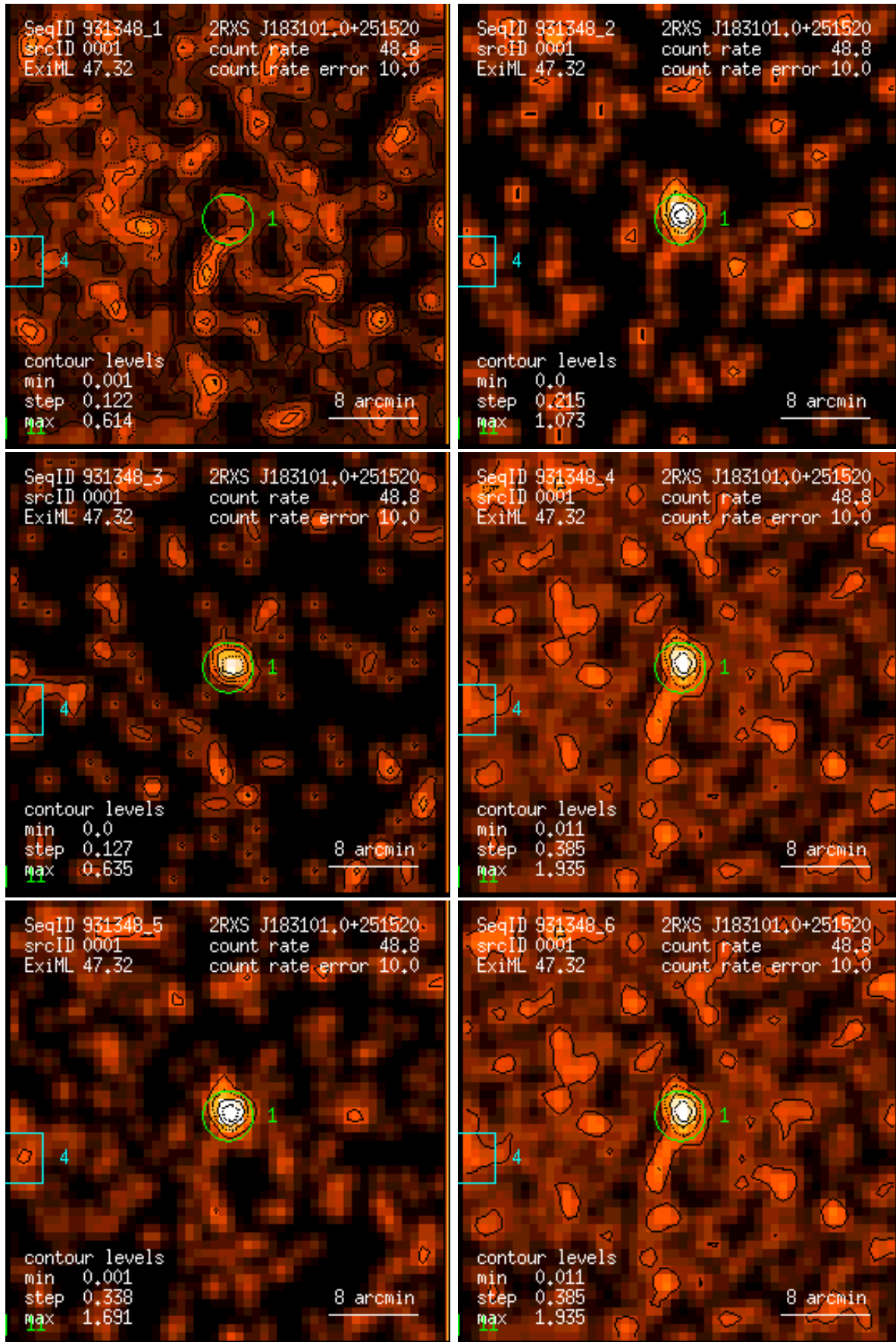
Figure 1: RASS 931348: detection 0001: band rate images, Gaussian filter: (1) PSPC channels 11 – 41, (2) 52 – 90, (3) 91 – 201, (4) 11 – 235, (5) 52 – 201, (6) 11 – 201. Broad band rates in counts/ks. Band rate contour levels in counts/ks/arcmin 2 .
