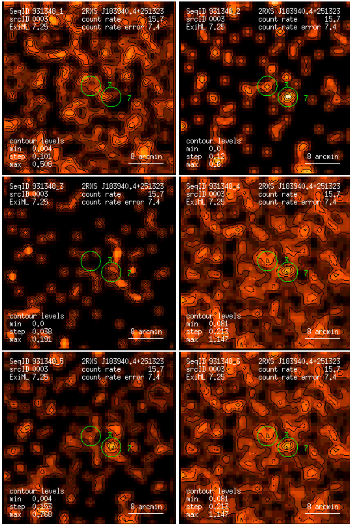
Figure 3: RASS 931348: detection 0003: band rate images, Gaussian filter: (1) PSPC channels 11 – 41, (2) 52 – 90, (3) 91 – 201, (4) 11 – 235, (5) 52 – 201, (6) 11 – 201. Broad band rates in counts/ks. Band rate contour levels in counts/ks/arcmin 2 .
