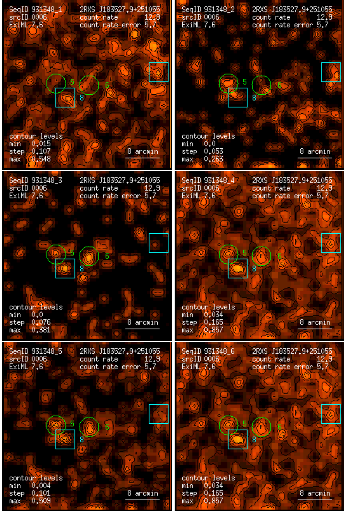
Figure 6: RASS 931348: detection 0006: band rate images, Gaussian filter: (1) PSPC channels 11 – 41, (2) 52 – 90, (3) 91 – 201, (4) 11 – 235, (5) 52 – 201, (6) 11 – 201. Broad band rates in counts/ks. Band rate contour levels in counts/ks/arcmin 2 .
