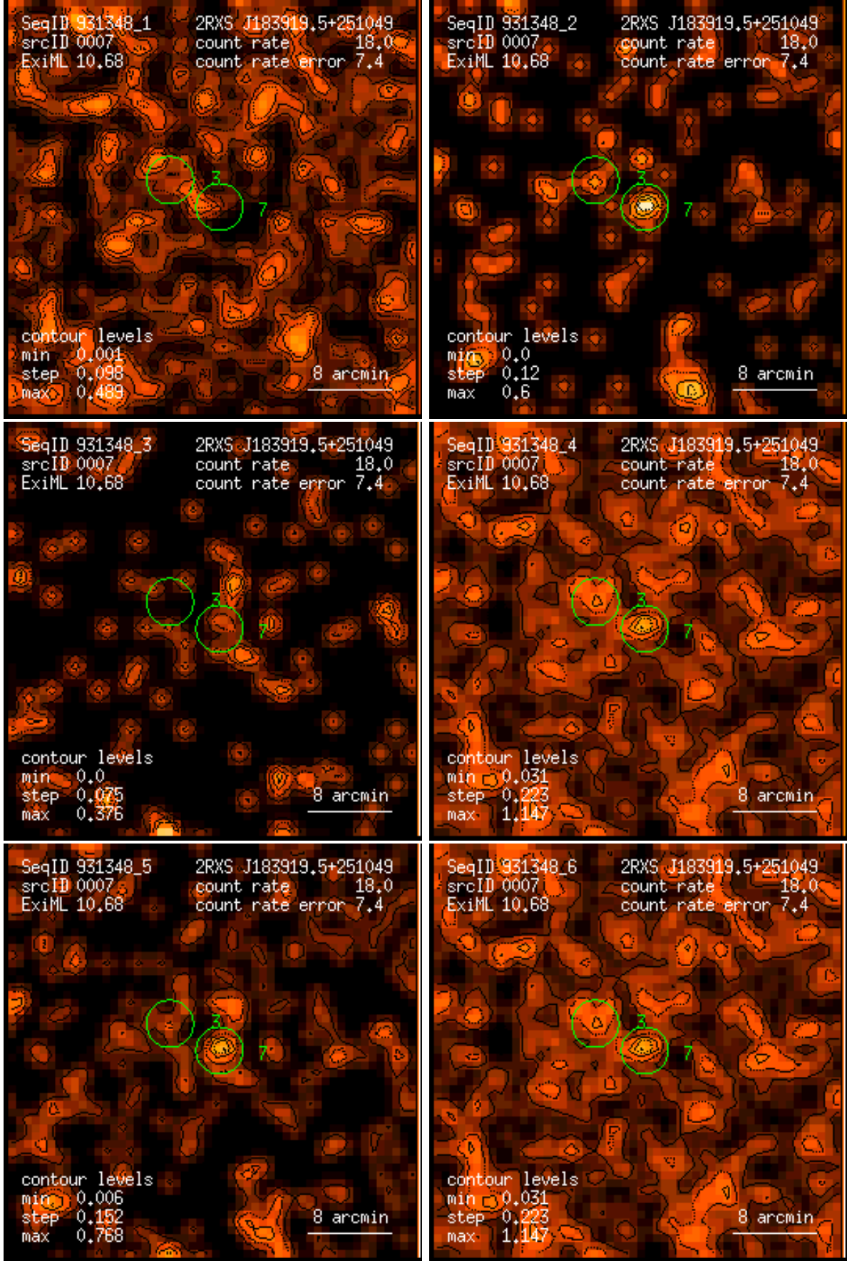
Figure 7: RASS 931348: detection 0007: band rate images, Gaussian filter: (1) PSPC channels 11 – 41, (2) 52 – 90, (3) 91 – 201, (4) 11 – 235, (5) 52 – 201, (6) 11 – 201. Broad band rates in counts/ks. Band rate contour levels in counts/ks/arcmin 2 .
