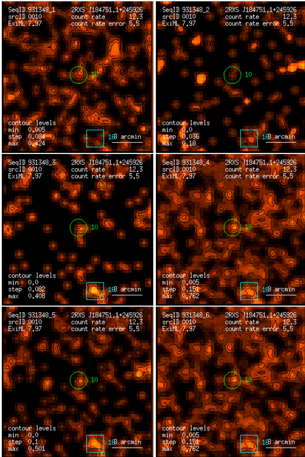
Figure 10: RASS 931348: detection 0010: band rate images, Gaussian filter: (1) PSPC channels 11 – 41, (2) 52 – 90, (3) 91 – 201, (4) 11 – 235, (5) 52 – 201, (6) 11 – 201. Broad band rates in counts/ks. Band rate contour levels in counts/ks/arcmin 2 .
