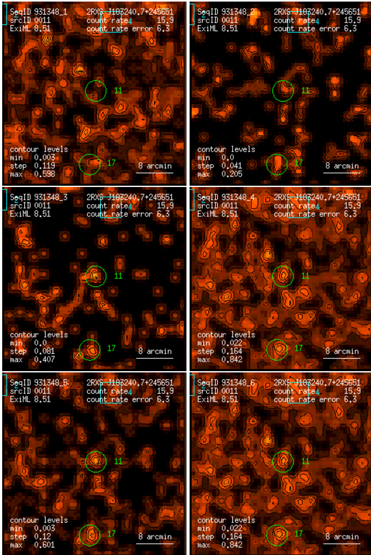
Figure 11: RASS 931348: detection 0011: band rate images, Gaussian filter: (1) PSPC channels 11 – 41, (2) 52 – 90, (3) 91 – 201, (4) 11 – 235, (5) 52 – 201, (6) 11 – 201. Broad band rates in counts/ks. Band rate contour levels in counts/ks/arcmin 2 .
