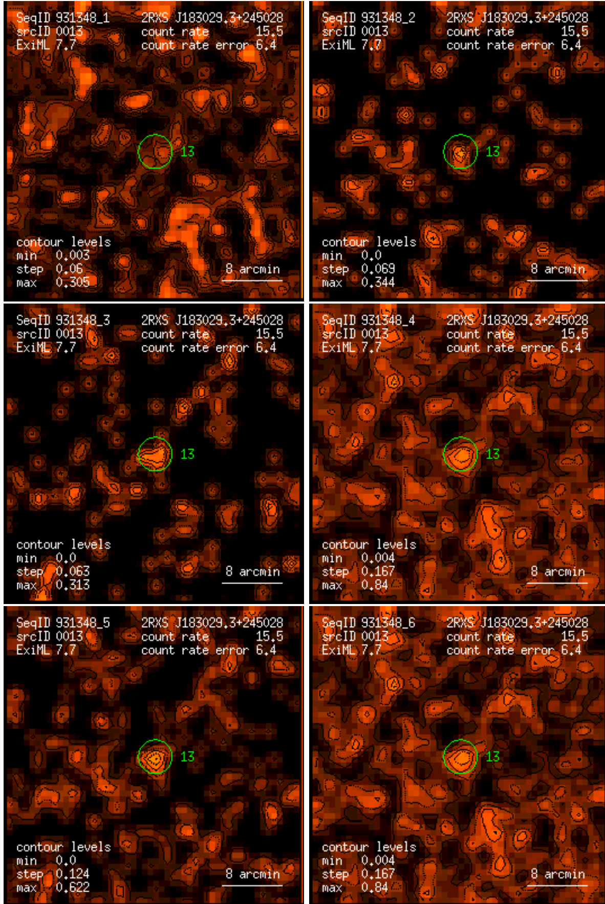
Figure 13: RASS 931348: detection 0013: band rate images, Gaussian filter: (1) PSPC channels 11 – 41, (2) 52 – 90, (3) 91 – 201, (4) 11 – 235, (5) 52 – 201, (6) 11 – 201. Broad band rates in counts/ks. Band rate contour levels in counts/ks/arcmin 2 .
