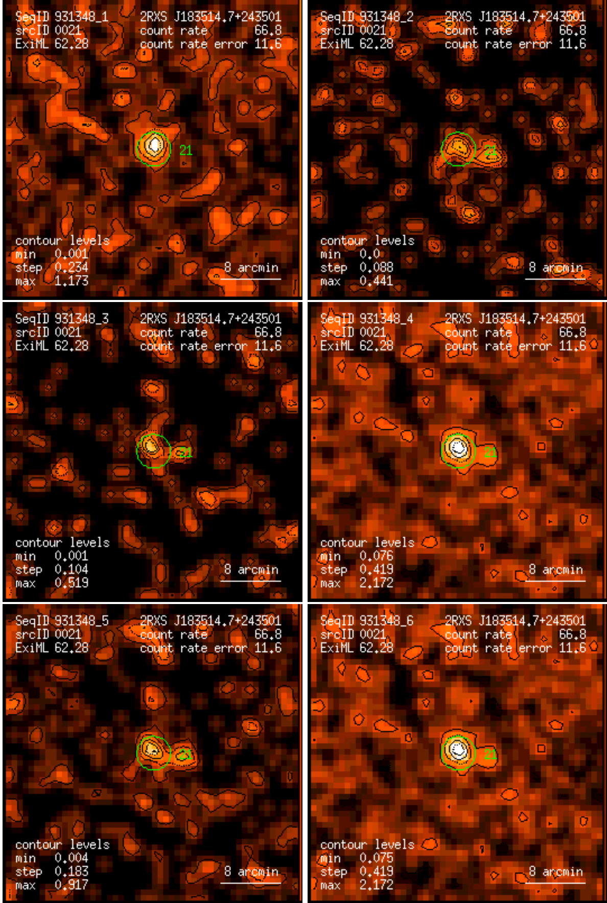
Figure 21: RASS 931348: detection 0021: band rate images, Gaussian filter: (1) PSPC channels 11 – 41, (2) 52 – 90, (3) 91 – 201, (4) 11 – 235, (5) 52 – 201, (6) 11 – 201. Broad band rates in counts/ks. Band rate contour levels in counts/ks/arcmin 2 .
