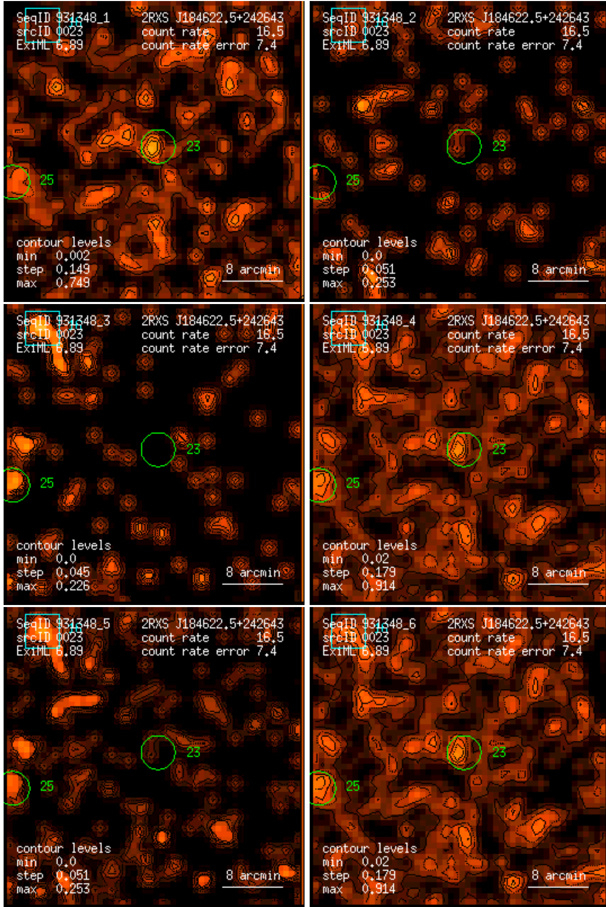
Figure 23: RASS 931348: detection 0023: band rate images, Gaussian filter: (1) PSPC channels 11 – 41, (2) 52 – 90, (3) 91 – 201, (4) 11 – 235, (5) 52 – 201, (6) 11 – 201. Broad band rates in counts/ks. Band rate contour levels in counts/ks/arcmin 2 .
