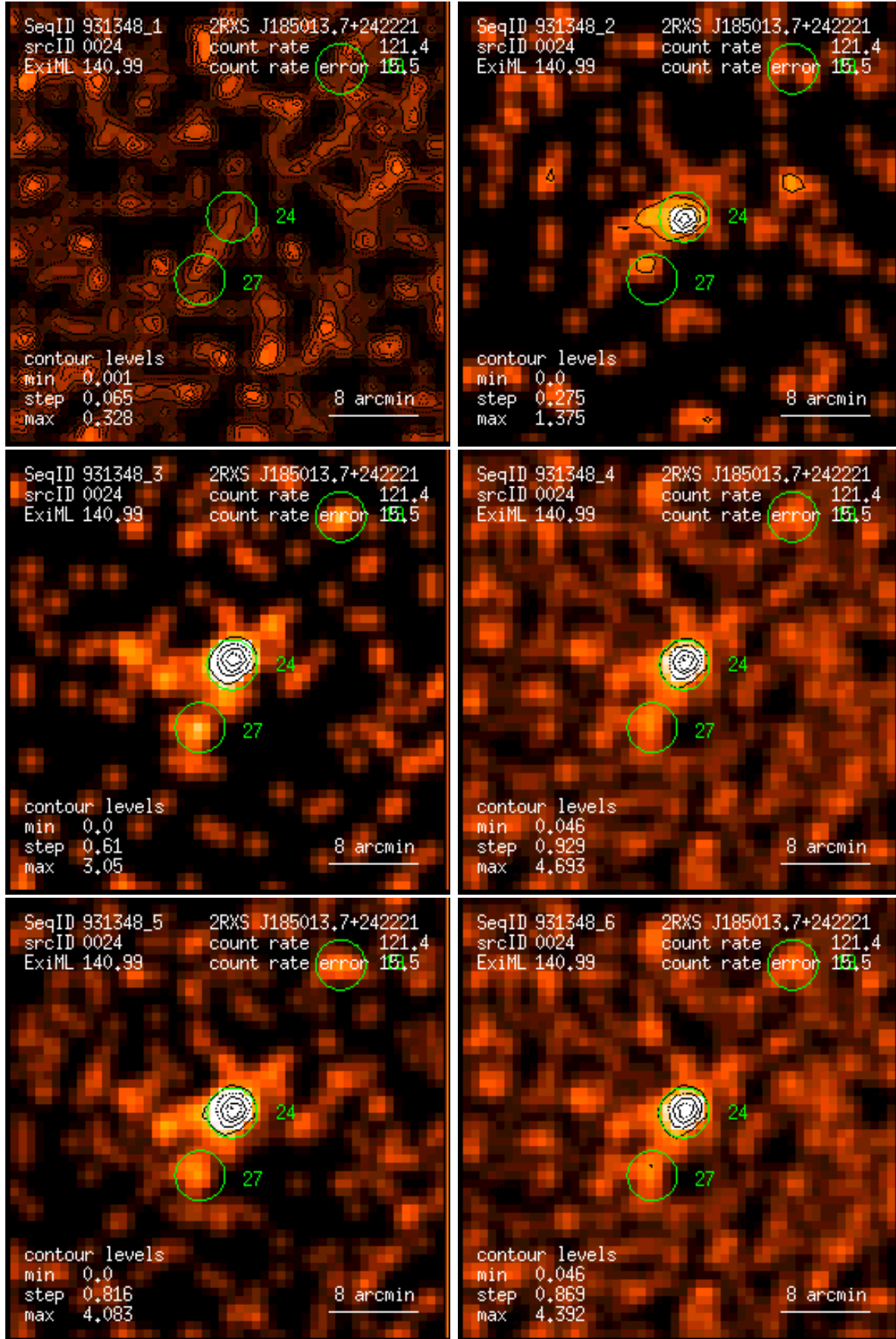
Figure 24: RASS 931348: detection 0024: band rate images, Gaussian filter: (1) PSPC channels 11 – 41, (2) 52 – 90, (3) 91 – 201, (4) 11 – 235, (5) 52 – 201, (6) 11 – 201. Broad band rates in counts/ks. Band rate contour levels in counts/ks/arcmin 2 .
