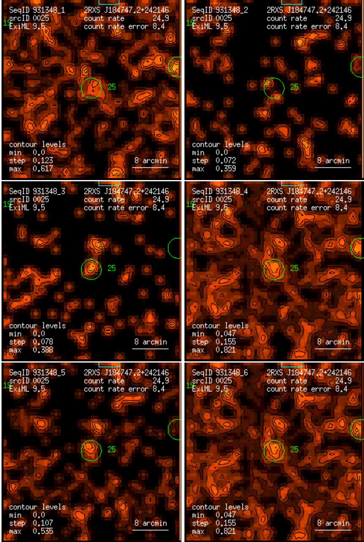
Figure 25: RASS 931348: detection 0025: band rate images, Gaussian filter: (1) PSPC channels 11 – 41, (2) 52 – 90, (3) 91 – 201, (4) 11 – 235, (5) 52 – 201, (6) 11 – 201. Broad band rates in counts/ks. Band rate contour levels in counts/ks/arcmin 2 .
