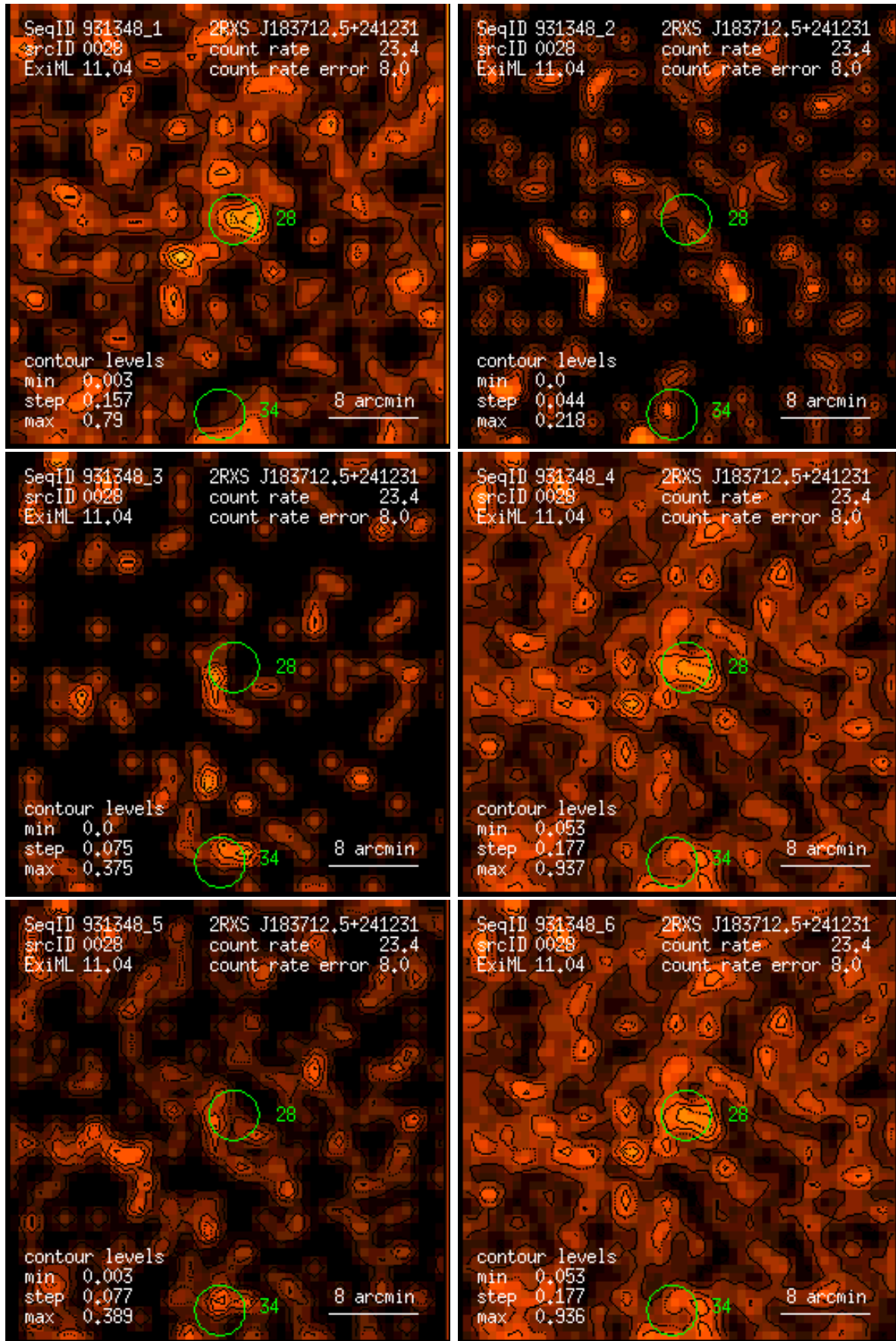
Figure 28: RASS 931348: detection 0028: band rate images, Gaussian filter: (1) PSPC channels 11 – 41, (2) 52 – 90, (3) 91 – 201, (4) 11 – 235, (5) 52 – 201, (6) 11 – 201. Broad band rates in counts/ks. Band rate contour levels in counts/ks/arcmin 2 .
