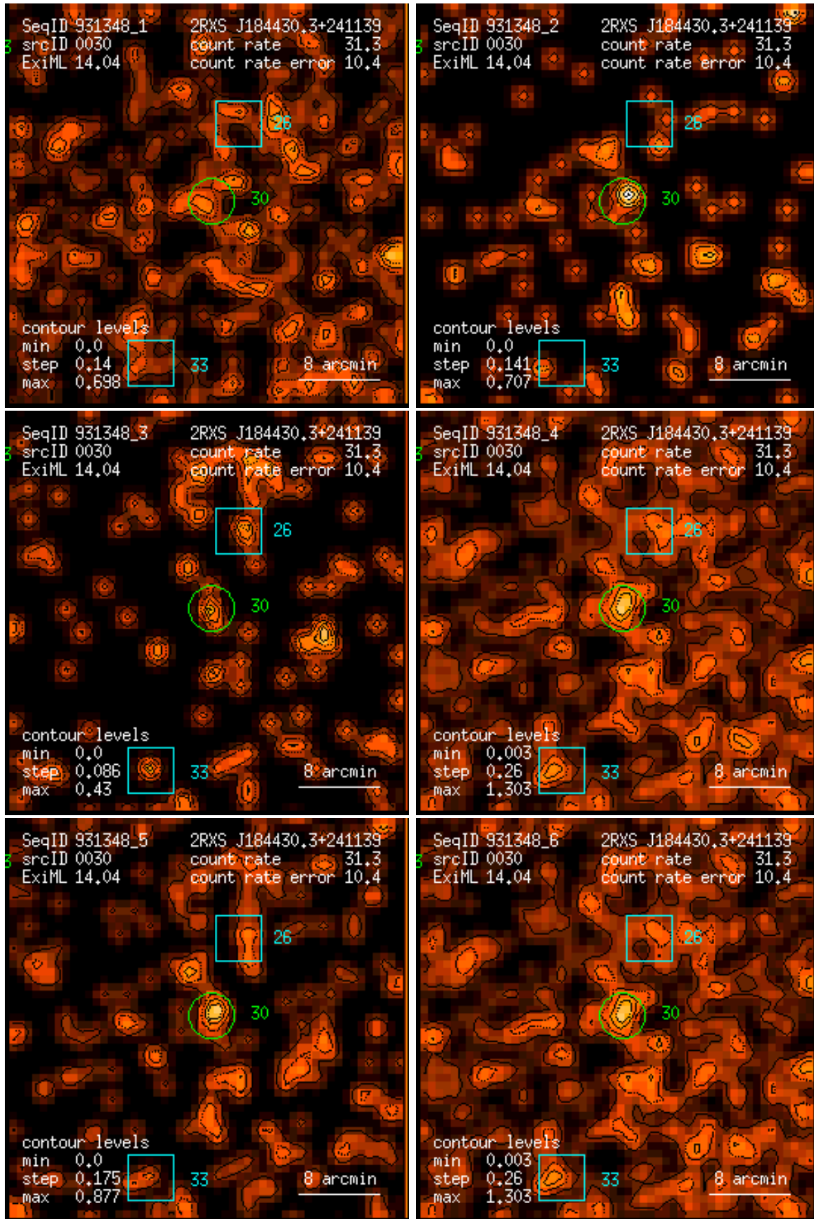
Figure 30: RASS 931348: detection 0030: band rate images, Gaussian filter: (1) PSPC channels 11 – 41, (2) 52 – 90, (3) 91 – 201, (4) 11 – 235, (5) 52 – 201, (6) 11 – 201. Broad band rates in counts/ks. Band rate contour levels in counts/ks/arcmin 2 .
