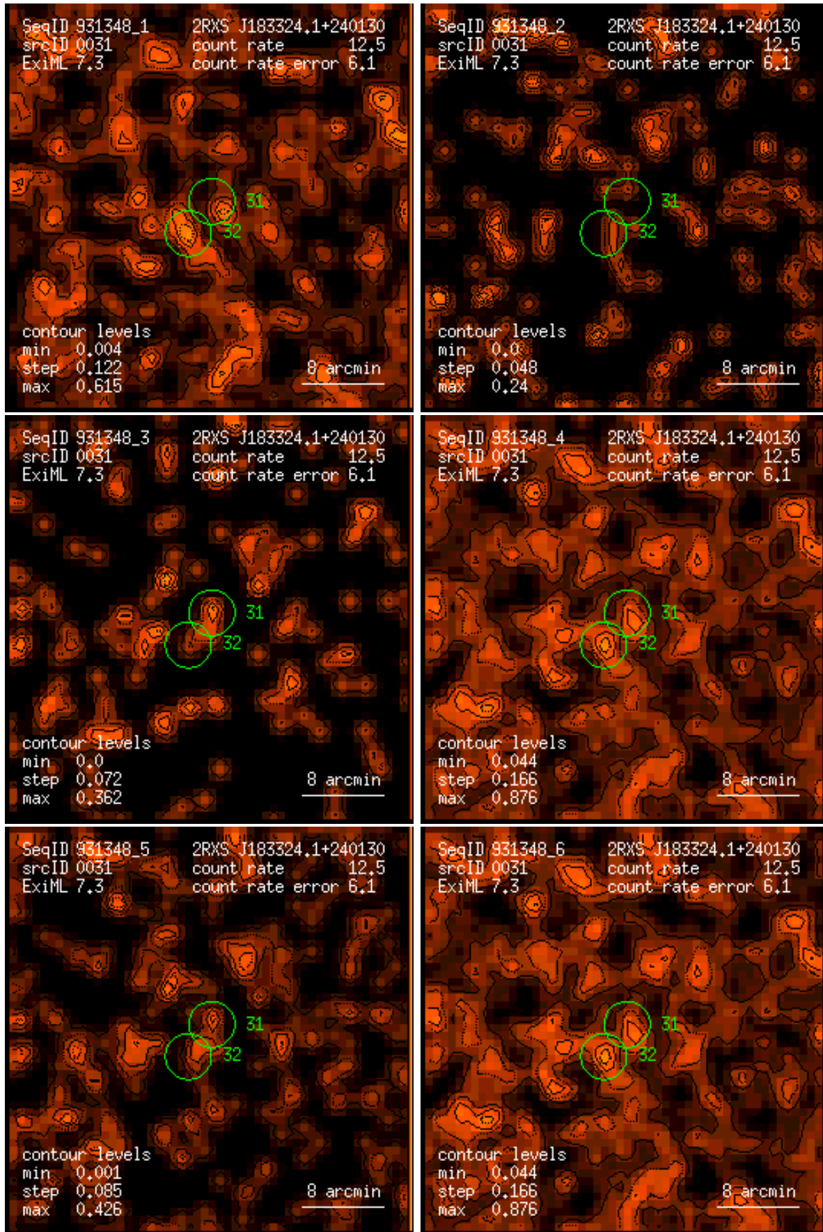
Figure 31: RASS 931348: detection 0031: band rate images, Gaussian filter: (1) PSPC channels 11 – 41, (2) 52 – 90, (3) 91 – 201, (4) 11 – 235, (5) 52 – 201, (6) 11 – 201. Broad band rates in counts/ks. Band rate contour levels in counts/ks/arcmin 2 .
