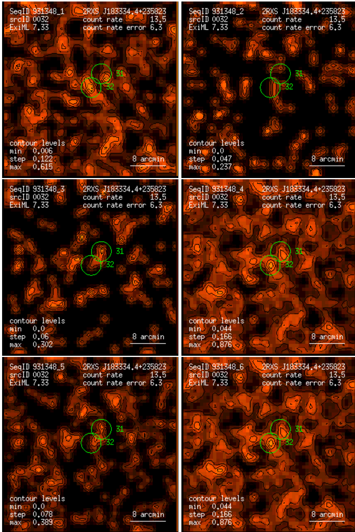
Figure 32: RASS 931348: detection 0032: band rate images, Gaussian filter: (1) PSPC channels 11 – 41, (2) 52 – 90, (3) 91 – 201, (4) 11 – 235, (5) 52 – 201, (6) 11 – 201. Broad band rates in counts/ks. Band rate contour levels in counts/ks/arcmin 2 .
