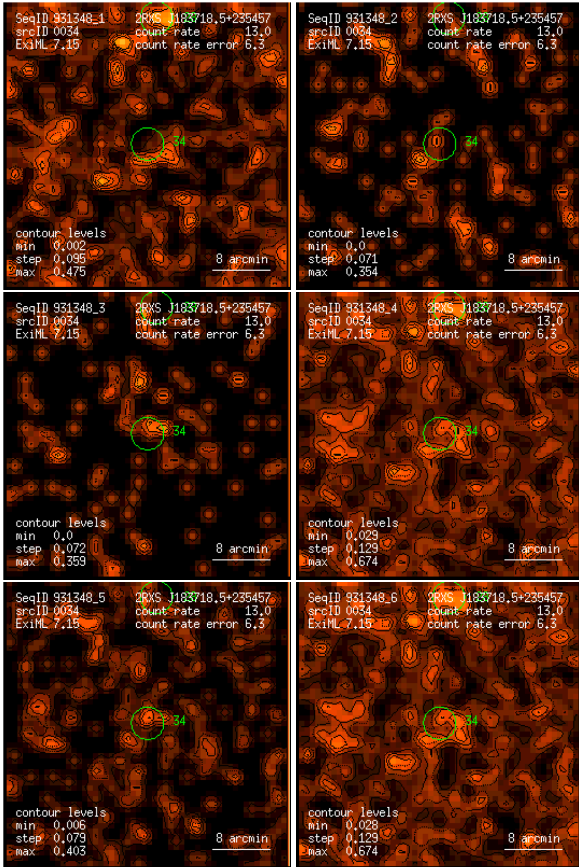
Figure 34: RASS 931348: detection 0034: band rate images, Gaussian filter: (1) PSPC channels 11 – 41, (2) 52 – 90, (3) 91 – 201, (4) 11 – 235, (5) 52 – 201, (6) 11 – 201. Broad band rates in counts/ks. Band rate contour levels in counts/ks/arcmin 2 .
