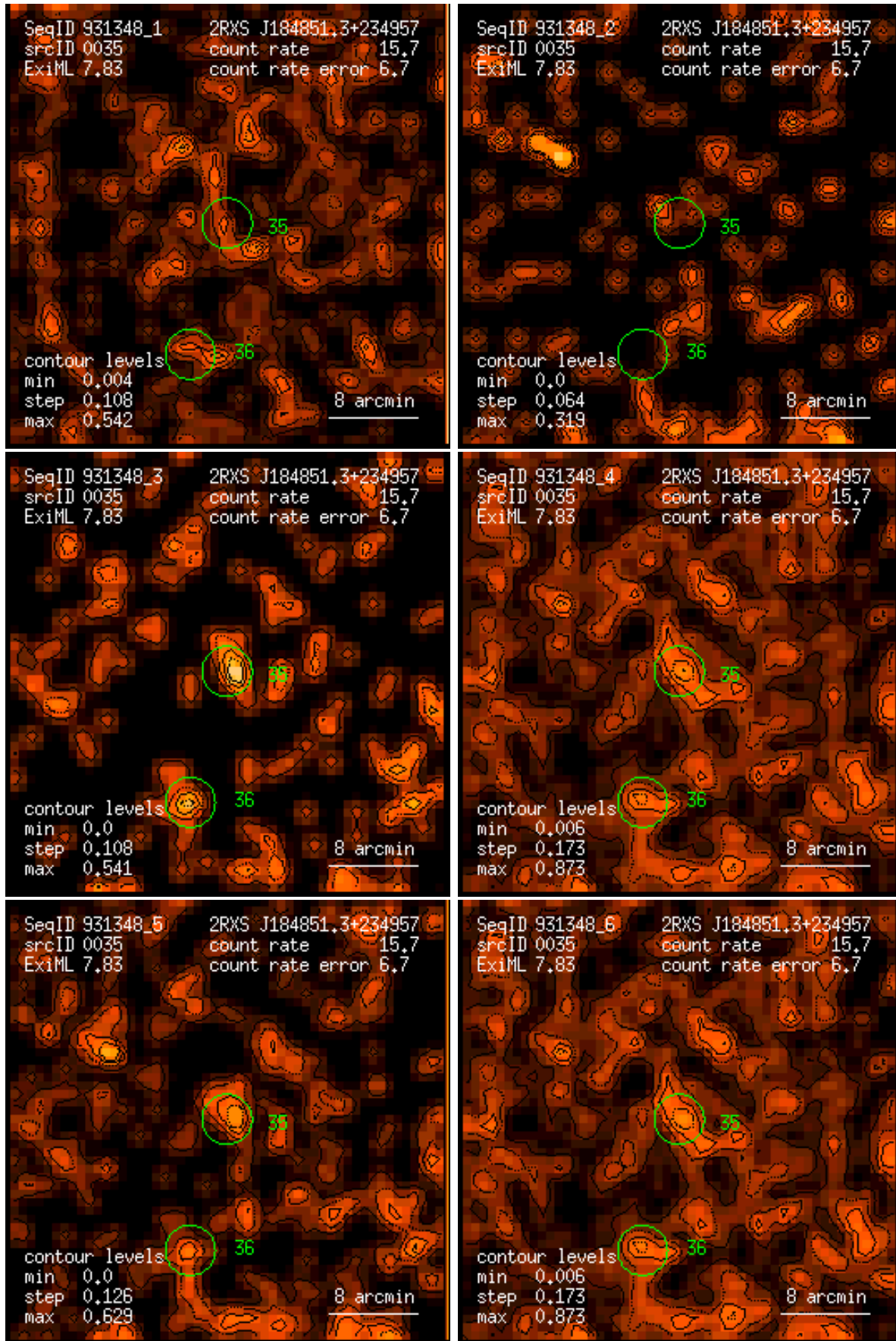
Figure 35: RASS 931348: detection 0035: band rate images, Gaussian filter: (1) PSPC channels 11 – 41, (2) 52 – 90, (3) 91 – 201, (4) 11 – 235, (5) 52 – 201, (6) 11 – 201. Broad band rates in counts/ks. Band rate contour levels in counts/ks/arcmin 2 .
