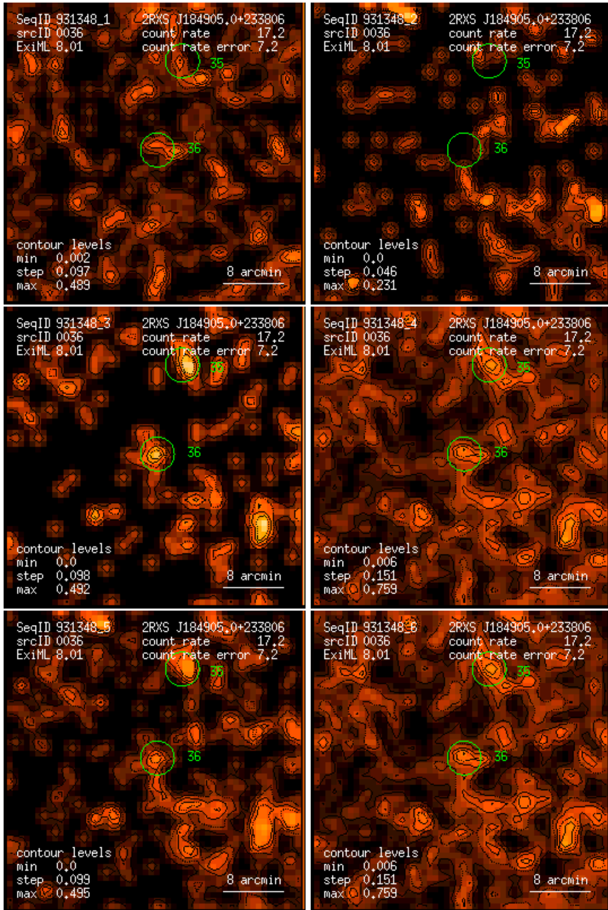
Figure 36: RASS 931348: detection 0036: band rate images, Gaussian filter: (1) PSPC channels 11 – 41, (2) 52 – 90, (3) 91 – 201, (4) 11 – 235, (5) 52 – 201, (6) 11 – 201. Broad band rates in counts/ks. Band rate contour levels in counts/ks/arcmin 2 .
