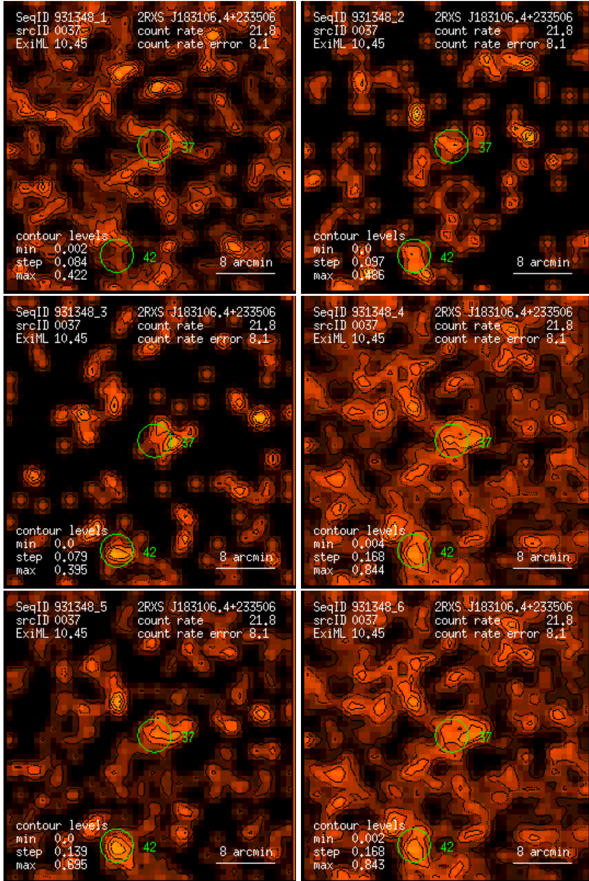
Figure 37: RASS 931348: detection 0037: band rate images, Gaussian filter: (1) PSPC channels 11 – 41, (2) 52 – 90, (3) 91 – 201, (4) 11 – 235, (5) 52 – 201, (6) 11 – 201. Broad band rates in counts/ks. Band rate contour levels in counts/ks/arcmin 2 .
