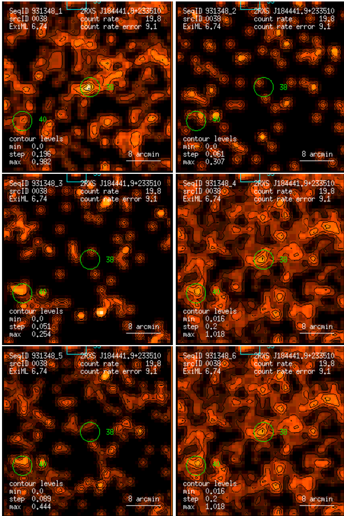
Figure 38: RASS 931348: detection 0038: band rate images, Gaussian filter: (1) PSPC channels 11 – 41, (2) 52 – 90, (3) 91 – 201, (4) 11 – 235, (5) 52 – 201, (6) 11 – 201. Broad band rates in counts/ks. Band rate contour levels in counts/ks/arcmin 2 .
