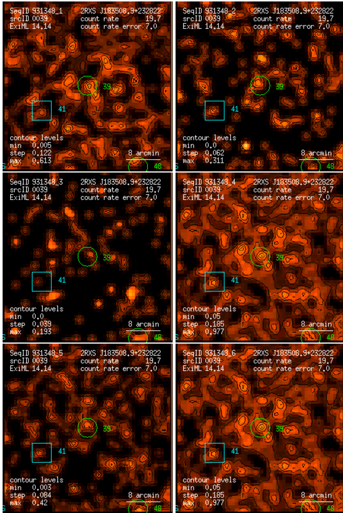
Figure 39: RASS 931348: detection 0039: band rate images, Gaussian filter: (1) PSPC channels 11 – 41, (2) 52 – 90, (3) 91 – 201, (4) 11 – 235, (5) 52 – 201, (6) 11 – 201. Broad band rates in counts/ks. Band rate contour levels in counts/ks/arcmin 2 .
