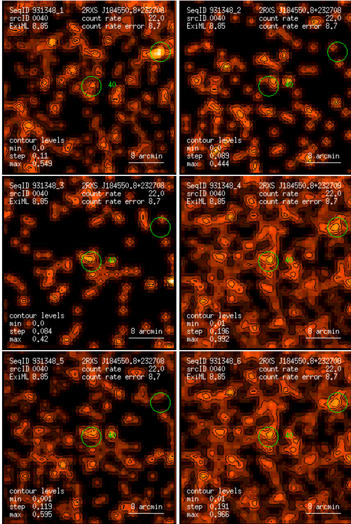
Figure 40: RASS 931348: detection 0040: band rate images, Gaussian filter: (1) PSPC channels 11 – 41, (2) 52 – 90, (3) 91 – 201, (4) 11 – 235, (5) 52 – 201, (6) 11 – 201. Broad band rates in counts/ks. Band rate contour levels in counts/ks/arcmin 2 .
