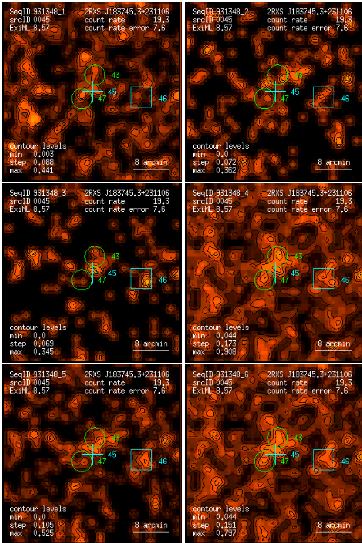
Figure 45: RASS 931348: detection 0045: band rate images, Gaussian filter: (1) PSPC channels 11 – 41, (2) 52 – 90, (3) 91 – 201, (4) 11 – 235, (5) 52 – 201, (6) 11 – 201. Broad band rates in counts/ks. Band rate contour levels in counts/ks/arcmin 2 .
