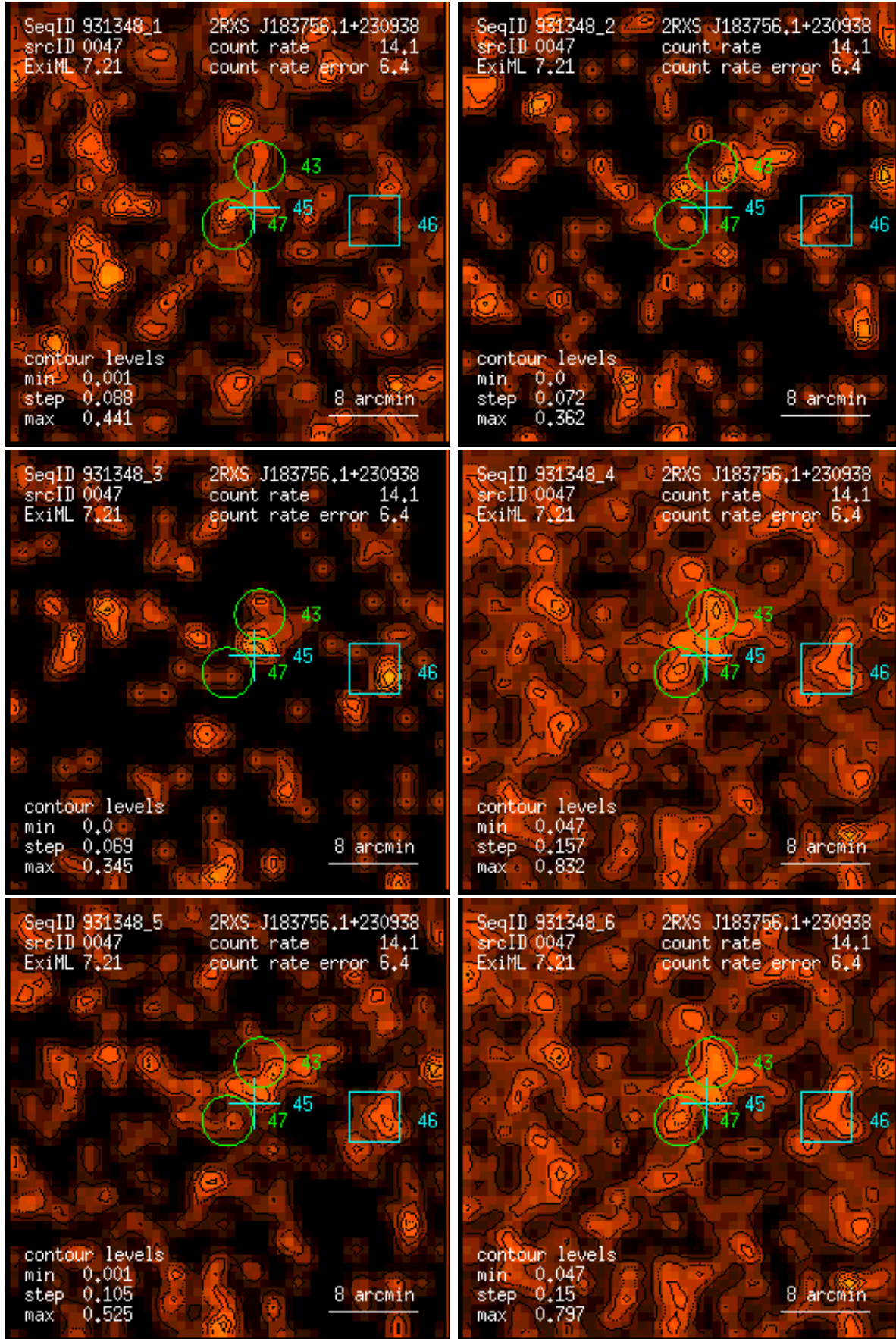
Figure 47: RASS 931348: detection 0047: band rate images, Gaussian filter: (1) PSPC channels 11 – 41, (2) 52 – 90, (3) 91 – 201, (4) 11 – 235, (5) 52 – 201, (6) 11 – 201. Broad band rates in counts/ks. Band rate contour levels in counts/ks/arcmin 2 .
