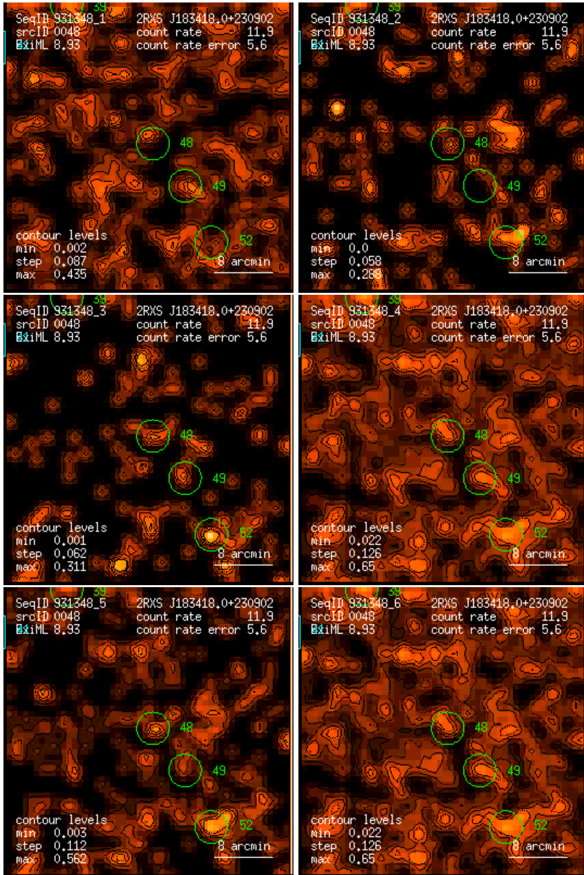
Figure 48: RASS 931348: detection 0048: band rate images, Gaussian filter: (1) PSPC channels 11 – 41, (2) 52 – 90, (3) 91 – 201, (4) 11 – 235, (5) 52 – 201, (6) 11 – 201. Broad band rates in counts/ks. Band rate contour levels in counts/ks/arcmin 2 .
