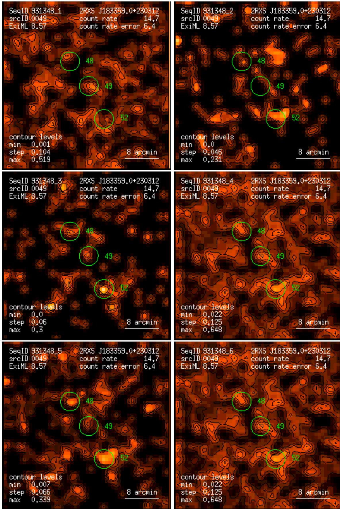
Figure 49: RASS 931348: detection 0049: band rate images, Gaussian filter: (1) PSPC channels 11 – 41, (2) 52 – 90, (3) 91 – 201, (4) 11 – 235, (5) 52 – 201, (6) 11 – 201. Broad band rates in counts/ks. Band rate contour levels in counts/ks/arcmin 2 .
