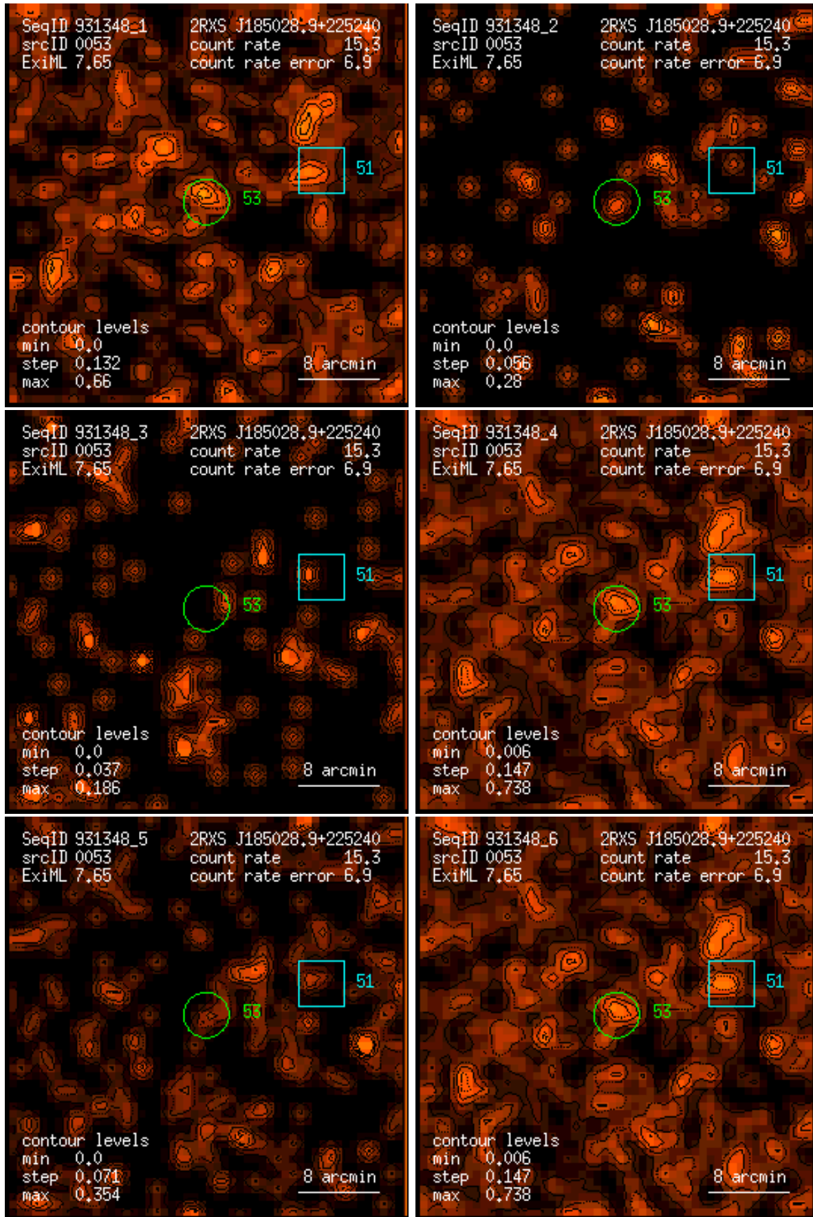
Figure 53: RASS 931348: detection 0053: band rate images, Gaussian filter: (1) PSPC channels 11 – 41, (2) 52 – 90, (3) 91 – 201, (4) 11 – 235, (5) 52 – 201, (6) 11 – 201. Broad band rates in counts/ks. Band rate contour levels in counts/ks/arcmin 2 .
