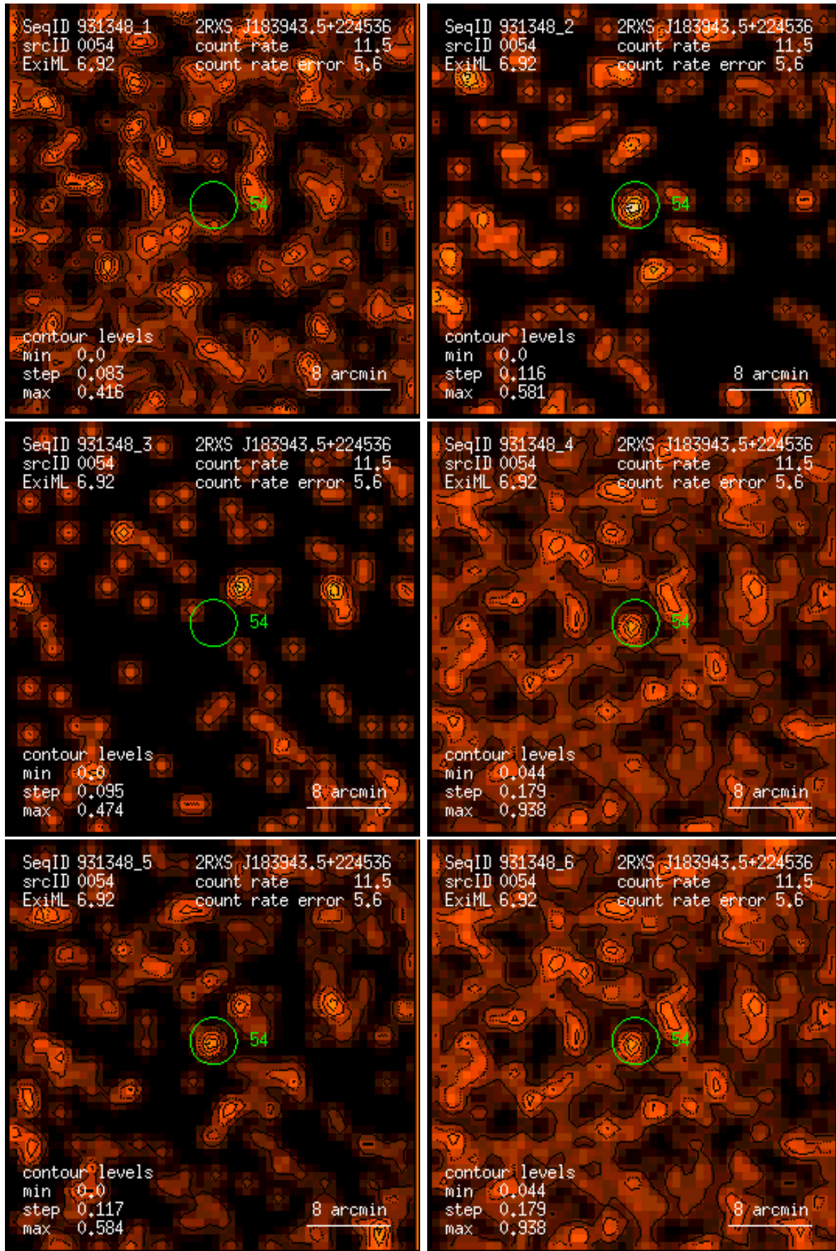
Figure 54: RASS 931348: detection 0054: band rate images, Gaussian filter: (1) PSPC channels 11 – 41, (2) 52 – 90, (3) 91 – 201, (4) 11 – 235, (5) 52 – 201, (6) 11 – 201. Broad band rates in counts/ks. Band rate contour levels in counts/ks/arcmin 2 .
