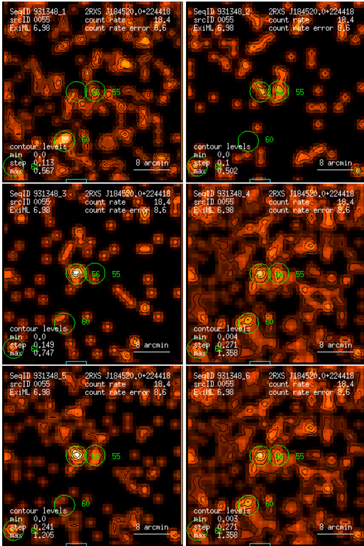
Figure 55: RASS 931348: detection 0055: band rate images, Gaussian filter: (1) PSPC channels 11 – 41, (2) 52 – 90, (3) 91 – 201, (4) 11 – 235, (5) 52 – 201, (6) 11 – 201. Broad band rates in counts/ks. Band rate contour levels in counts/ks/arcmin 2 .
