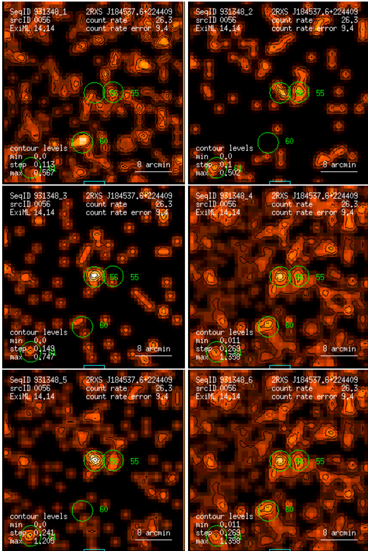
Figure 56: RASS 931348: detection 0056: band rate images, Gaussian filter: (1) PSPC channels 11 – 41, (2) 52 – 90, (3) 91 – 201, (4) 11 – 235, (5) 52 – 201, (6) 11 – 201. Broad band rates in counts/ks. Band rate contour levels in counts/ks/arcmin 2 .
