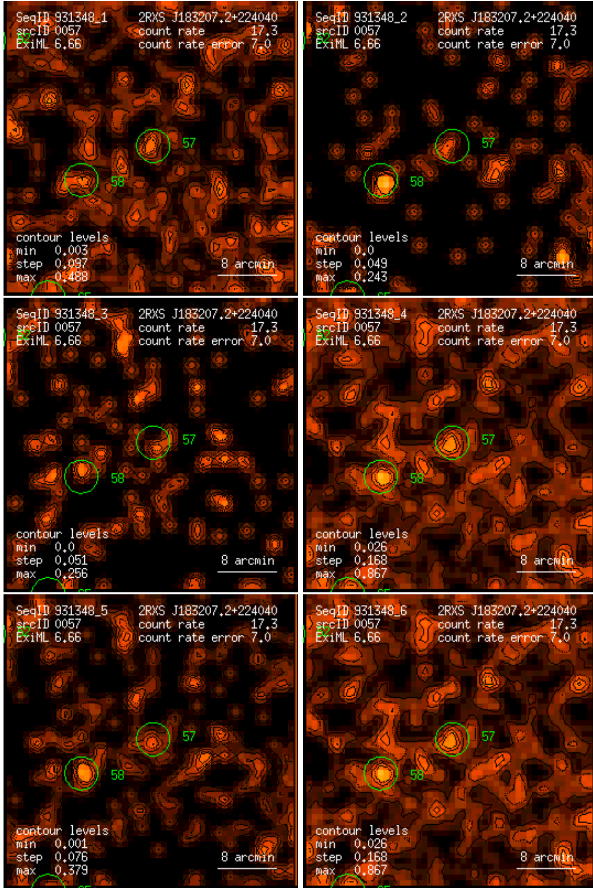
Figure 57: RASS 931348: detection 0057: band rate images, Gaussian filter: (1) PSPC channels 11 – 41, (2) 52 – 90, (3) 91 – 201, (4) 11 – 235, (5) 52 – 201, (6) 11 – 201. Broad band rates in counts/ks. Band rate contour levels in counts/ks/arcmin 2 .
