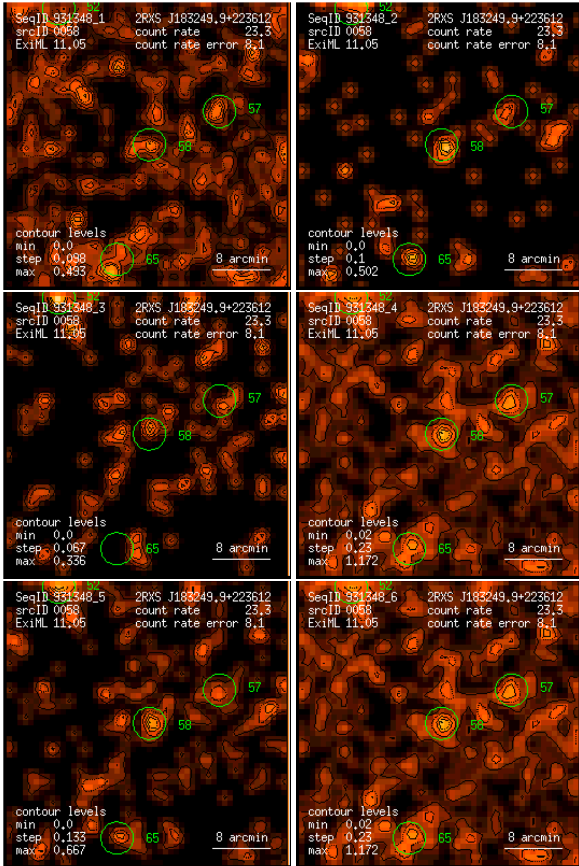
Figure 58: RASS 931348: detection 0058: band rate images, Gaussian filter: (1) PSPC channels 11 – 41, (2) 52 – 90, (3) 91 – 201, (4) 11 – 235, (5) 52 – 201, (6) 11 – 201. Broad band rates in counts/ks. Band rate contour levels in counts/ks/arcmin 2 .
