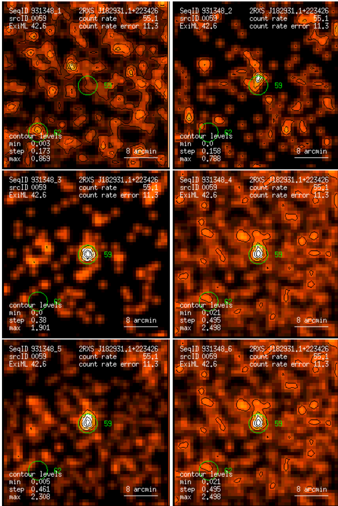
Figure 59: RASS 931348: detection 0059: band rate images, Gaussian filter: (1) PSPC channels 11 – 41, (2) 52 – 90, (3) 91 – 201, (4) 11 – 235, (5) 52 – 201, (6) 11 – 201. Broad band rates in counts/ks. Band rate contour levels in counts/ks/arcmin 2 .
