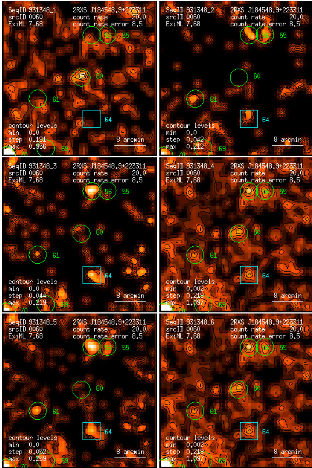
Figure 60: RASS 931348: detection 0060: band rate images, Gaussian filter: (1) PSPC channels 11 – 41, (2) 52 – 90, (3) 91 – 201, (4) 11 – 235, (5) 52 – 201, (6) 11 – 201. Broad band rates in counts/ks. Band rate contour levels in counts/ks/arcmin 2 .
