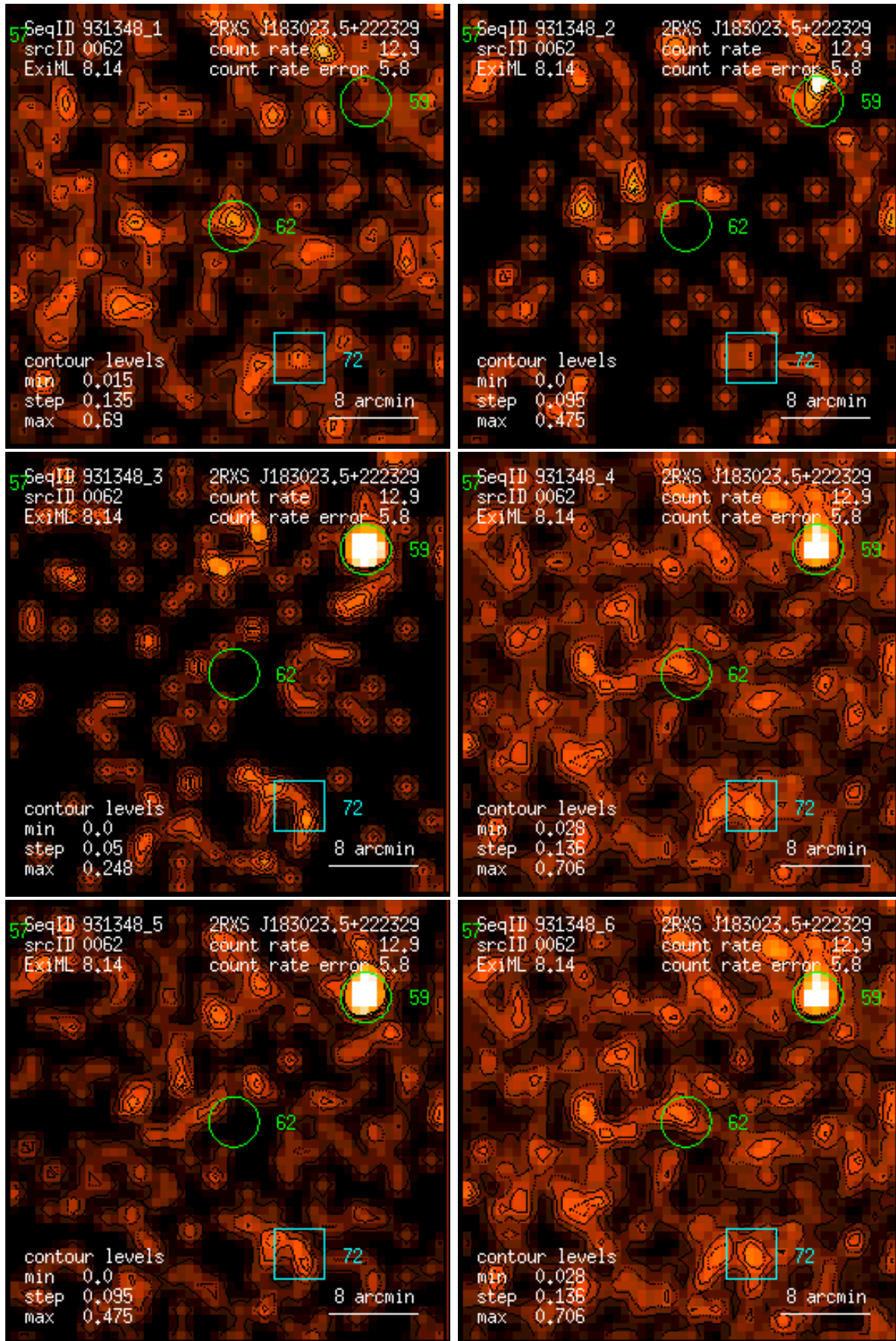
Figure 62: RASS 931348: detection 0062: band rate images, Gaussian filter: (1) PSPC channels 11 – 41, (2) 52 – 90, (3) 91 – 201, (4) 11 – 235, (5) 52 – 201, (6) 11 – 201. Broad band rates in counts/ks. Band rate contour levels in counts/ks/arcmin 2 .
