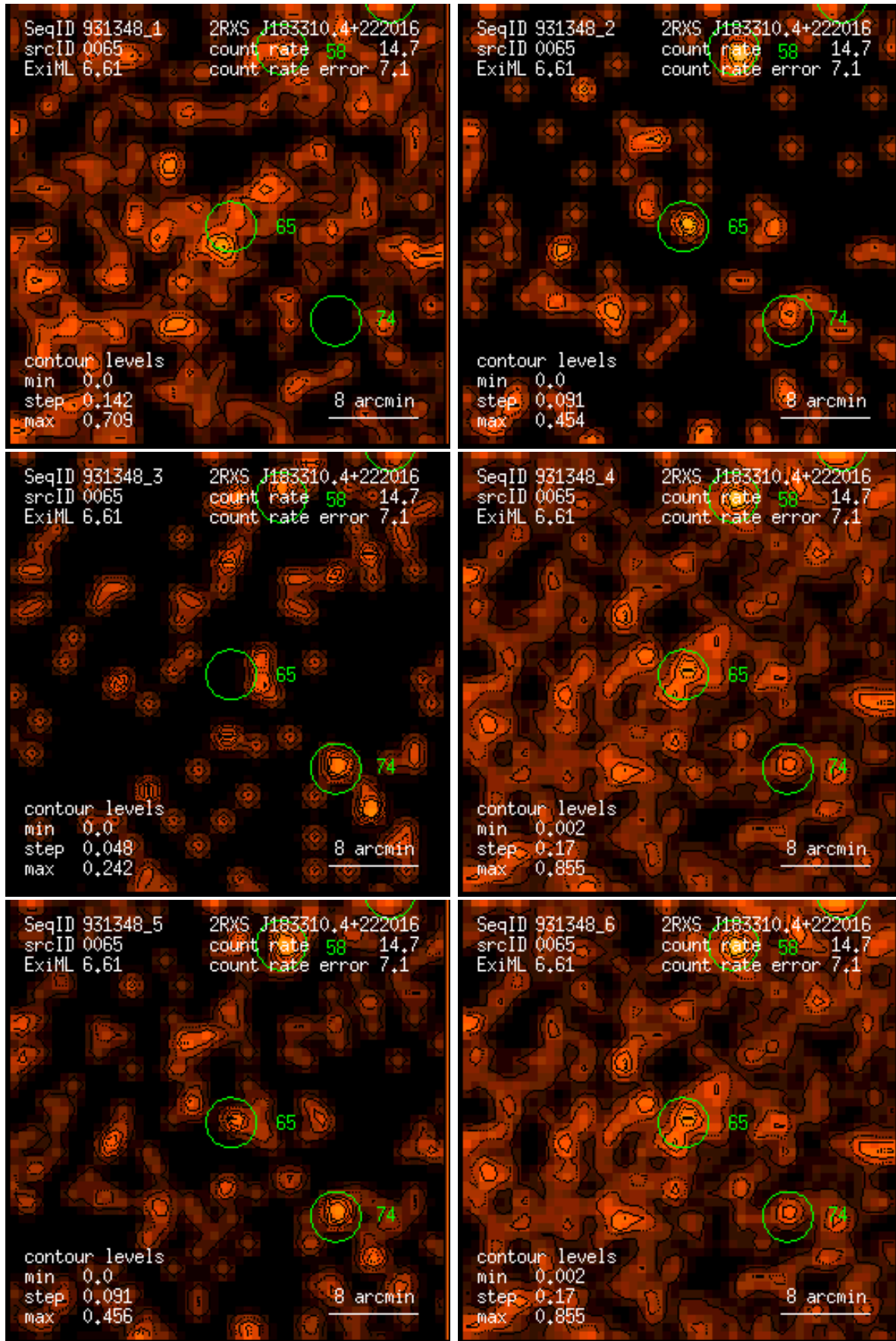
Figure 65: RASS 931348: detection 0065: band rate images, Gaussian filter: (1) PSPC channels 11 – 41, (2) 52 – 90, (3) 91 – 201, (4) 11 – 235, (5) 52 – 201, (6) 11 – 201. Broad band rates in counts/ks. Band rate contour levels in counts/ks/arcmin 2 .
