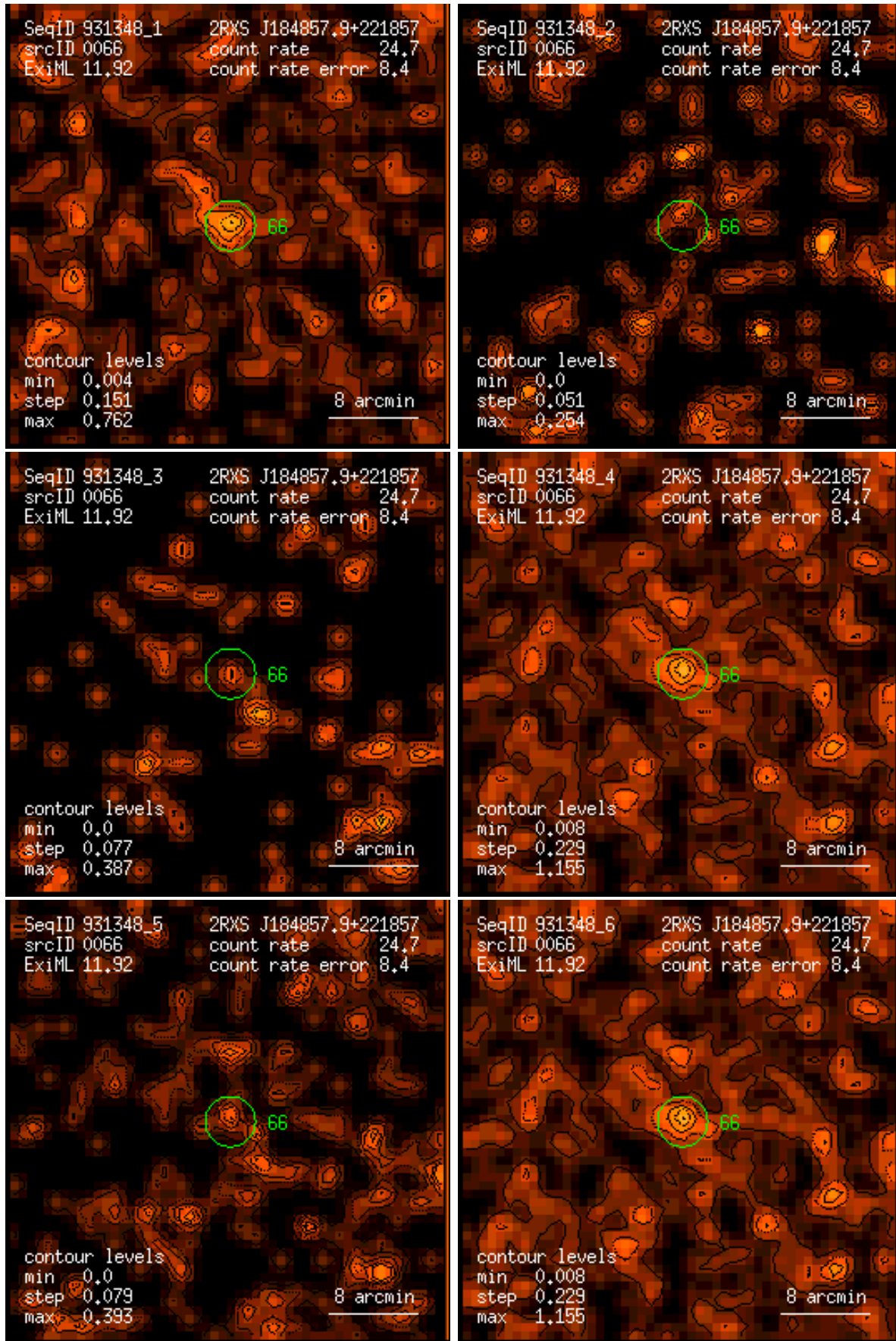
Figure 66: RASS 931348: detection 0066: band rate images, Gaussian filter: (1) PSPC channels 11 – 41, (2) 52 – 90, (3) 91 – 201, (4) 11 – 235, (5) 52 – 201, (6) 11 – 201. Broad band rates in counts/ks. Band rate contour levels in counts/ks/arcmin 2 .
