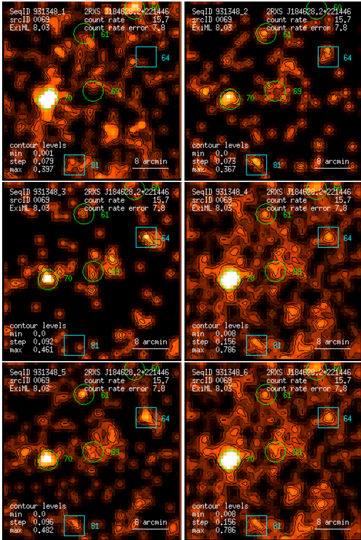
Figure 69: RASS 931348: detection 0069: band rate images, Gaussian filter: (1) PSPC channels 11 – 41, (2) 52 – 90, (3) 91 – 201, (4) 11 – 235, (5) 52 – 201, (6) 11 – 201. Broad band rates in counts/ks. Band rate contour levels in counts/ks/arcmin 2 .
