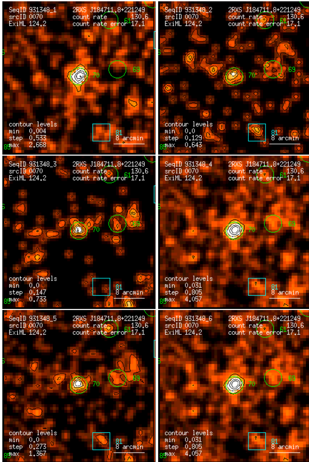
Figure 70: RASS 931348: detection 0070: band rate images, Gaussian filter: (1) PSPC channels 11 – 41, (2) 52 – 90, (3) 91 – 201, (4) 11 – 235, (5) 52 – 201, (6) 11 – 201. Broad band rates in counts/ks. Band rate contour levels in counts/ks/arcmin 2 .
