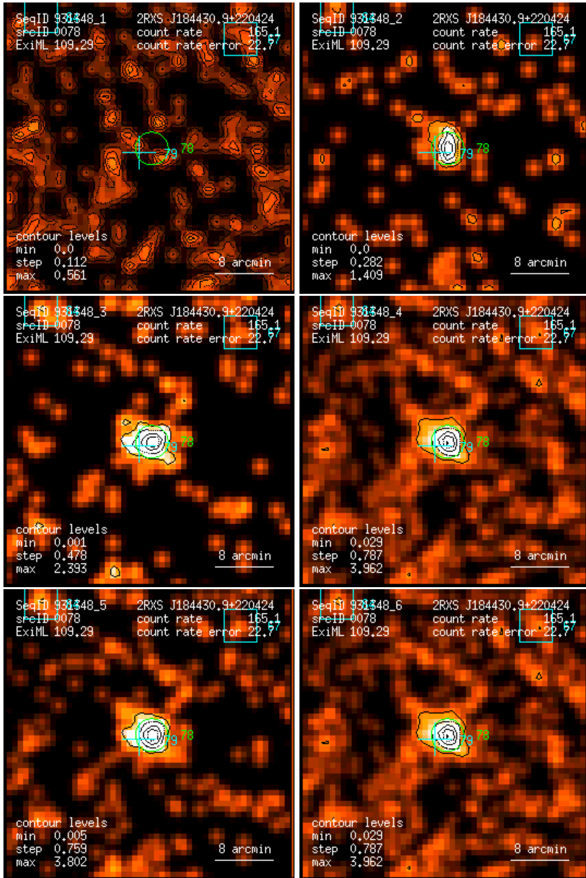
Figure 78: RASS 931348: detection 0078: band rate images, Gaussian filter: (1) PSPC channels 11 – 41, (2) 52 – 90, (3) 91 – 201, (4) 11 – 235, (5) 52 – 201, (6) 11 – 201. Broad band rates in counts/ks. Band rate contour levels in counts/ks/arcmin 2 .
