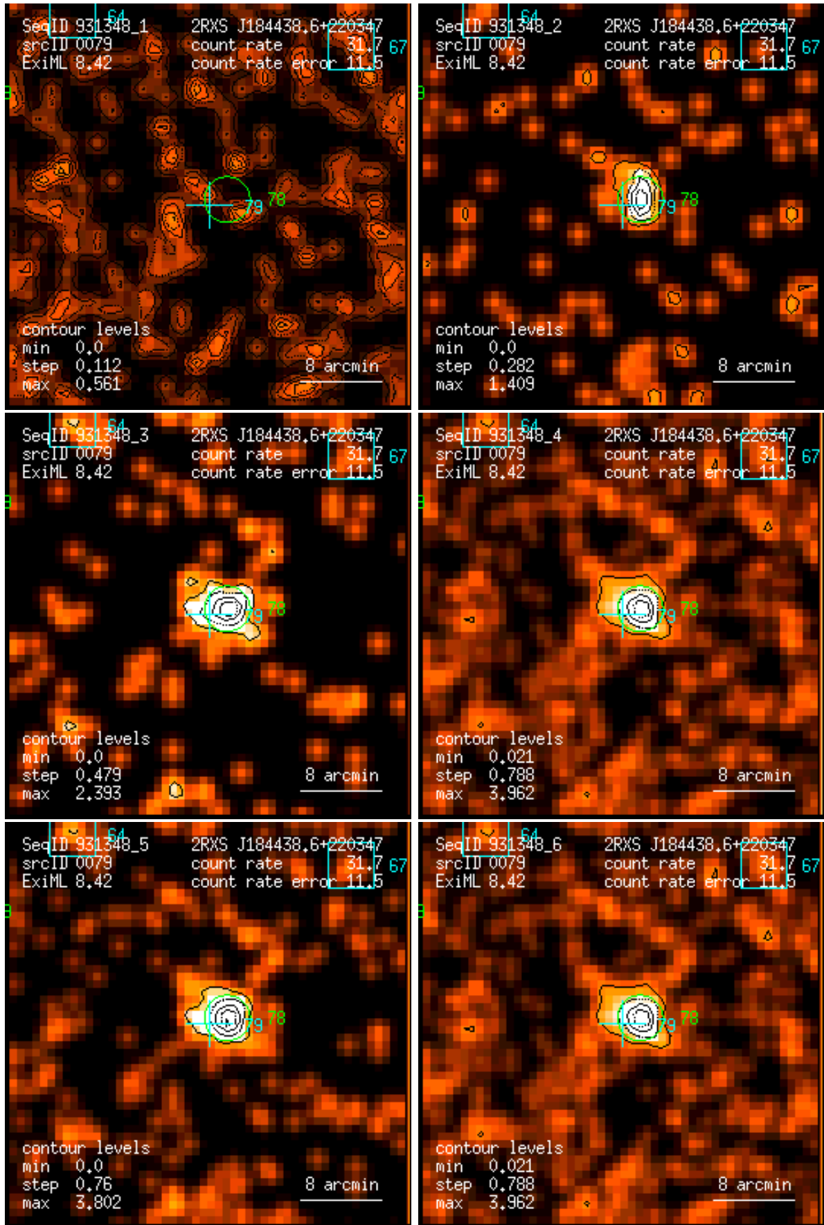
Figure 79: RASS 931348: detection 0079: band rate images, Gaussian filter: (1) PSPC channels 11 – 41, (2) 52 – 90, (3) 91 – 201, (4) 11 – 235, (5) 52 – 201, (6) 11 – 201. Broad band rates in counts/ks. Band rate contour levels in counts/ks/arcmin 2 .
